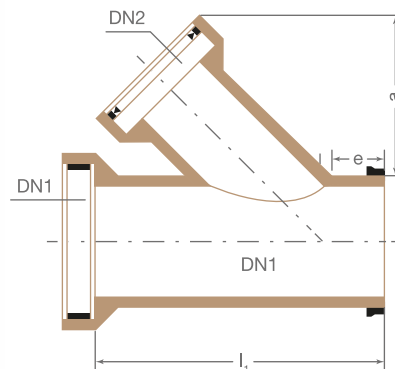
Aftakking 45°
